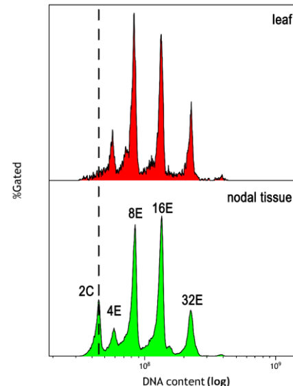
Figure 5. DNA histograms from Vanilla planifolia somatic tissues. Here, the X-axis is logarithmic. Note that euploid nuclei are sometimes difficult to assess in leaf, complicating the estimations of genome-size and of the endoreplication process itself. Contrastingly, in nodal tissue, the 2C nuclei, essential for assessing genome size, constituted exceptionally a fifth of this sample of orchid nuclei. Populations of larger nuclei were also evident: 4E, 8E, 16E, 32E, and a trace of 64E. E is the quantity of DNA association with a single genome undergoing endoreplication.
