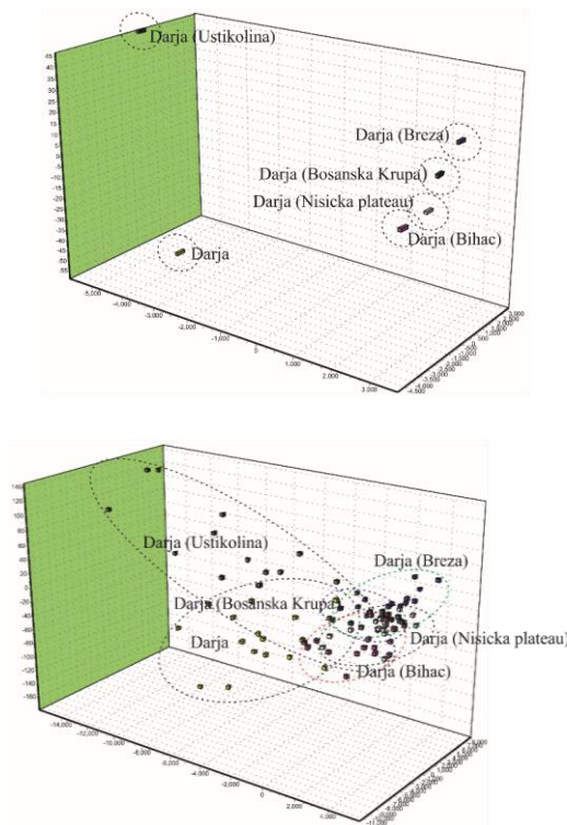
Figure 1. Multivariate analysis (Factorial Correspondence Analysis - FCA) of simple sequence repeat data for the reference and analyzed samples of 'Darja'- sample centroids (above) and individuals (beneath) shown
